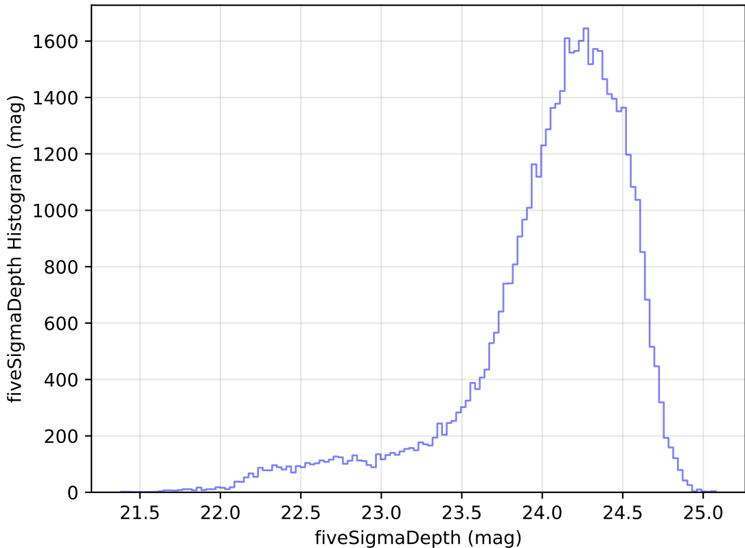
too_elab_r16_d3_gz_v3.4_10yrs Yr 1 r band: fiveSigmaDepth Histogram
