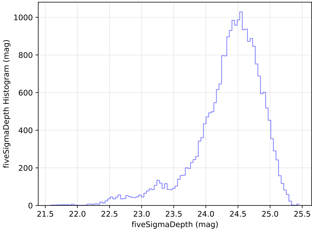
too_elab_r16_d3_gz_v3.4_10yrs Yr 1 g band: fiveSigmaDepth Histogram
