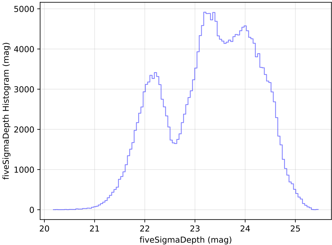
too_elab_r16_d3_gz_v3.4_10yrs Yr 1 all bands: fiveSigmaDepth Histogram
