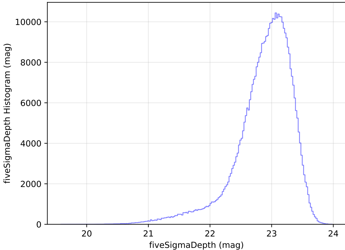
too_elab_r16_d3_gz_v3.4_10yrs WFD z band: fiveSigmaDepth Histogram
