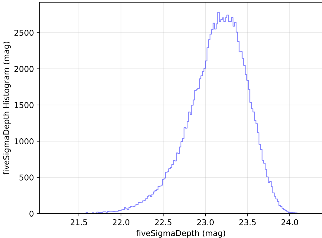
too_elab_r16_d3_gz_v3.4_10yrs WFD u band: fiveSigmaDepth Histogram
