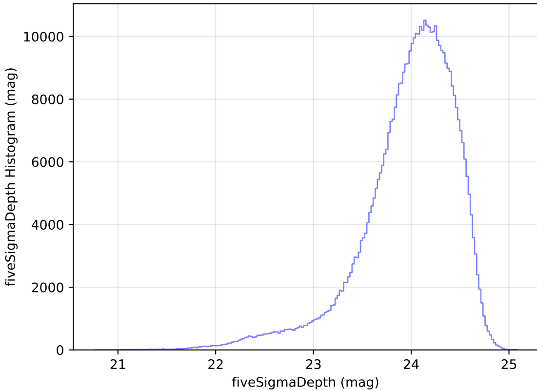
too_elab_r16_d3_gz_v3.4_10yrs WFD r band: fiveSigmaDepth Histogram
