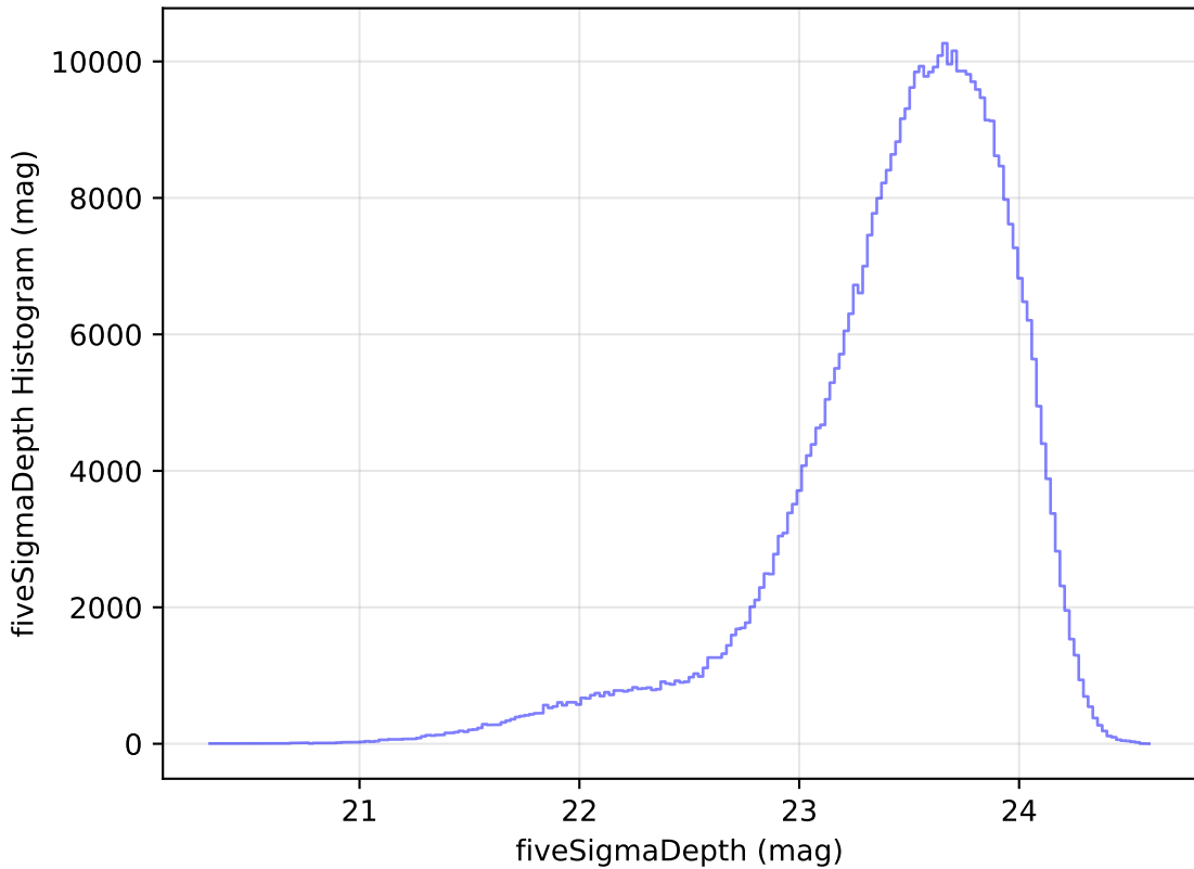
too_elab_r16_d3_gz_v3.4_10yrs WFD i band: fiveSigmaDepth Histogram
