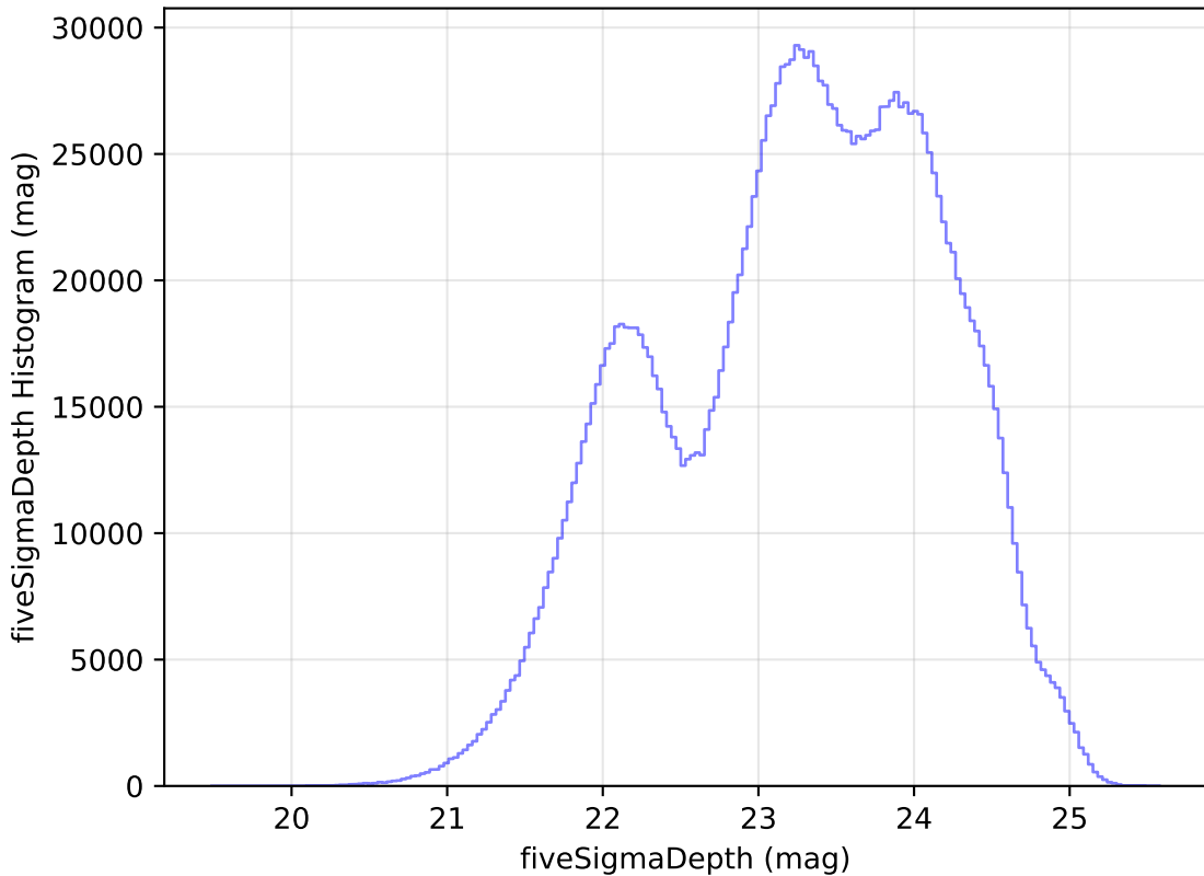
too_elab_r16_d3_gz_v3.4_10yrs WFD all bands: fiveSigmaDepth Histogram
