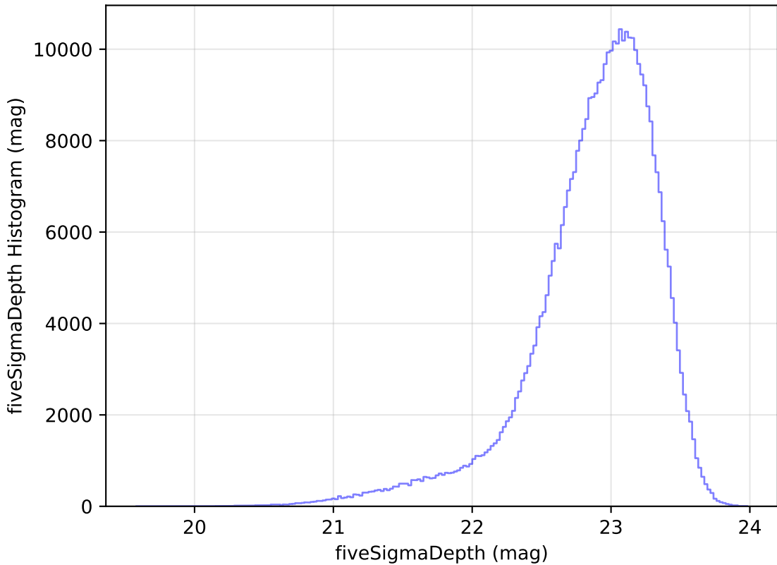
too_elab_r16_d3_gz_v3.4_10yrs All sky z band: fiveSigmaDepth Histogram
