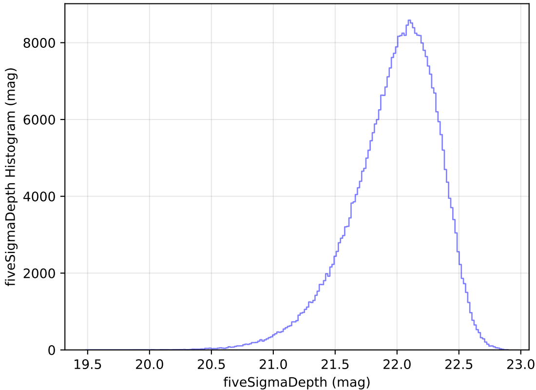
too_elab_r16_d3_gz_v3.4_10yrs All sky y band: fiveSigmaDepth Histogram
