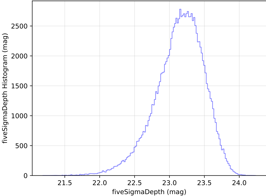
too_elab_r16_d3_gz_v3.4_10yrs All sky u band: fiveSigmaDepth Histogram
