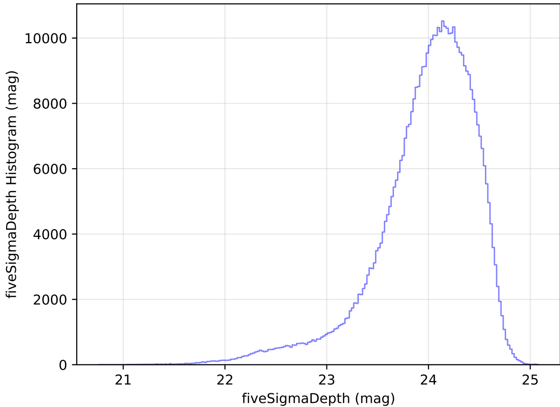
too_elab_r16_d3_gz_v3.4_10yrs All sky r band: fiveSigmaDepth Histogram
