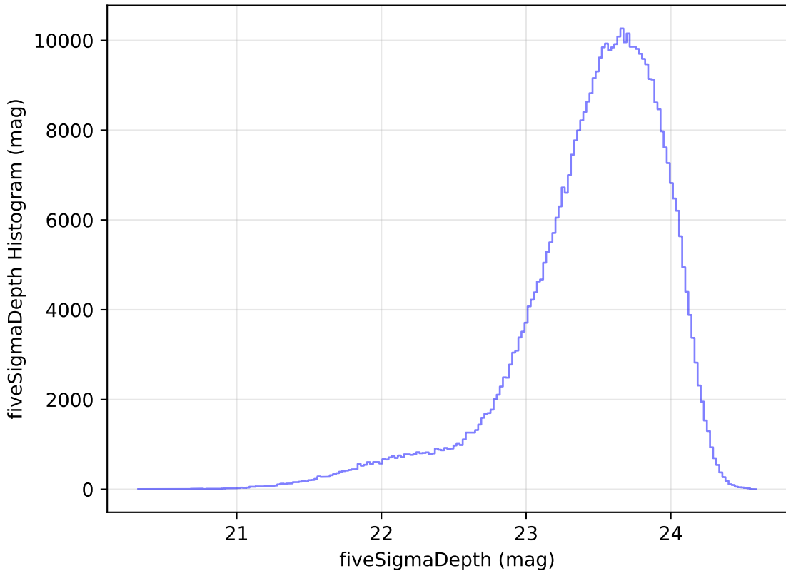
too_elab_r16_d3_gz_v3.4_10yrs All sky i band: fiveSigmaDepth Histogram
