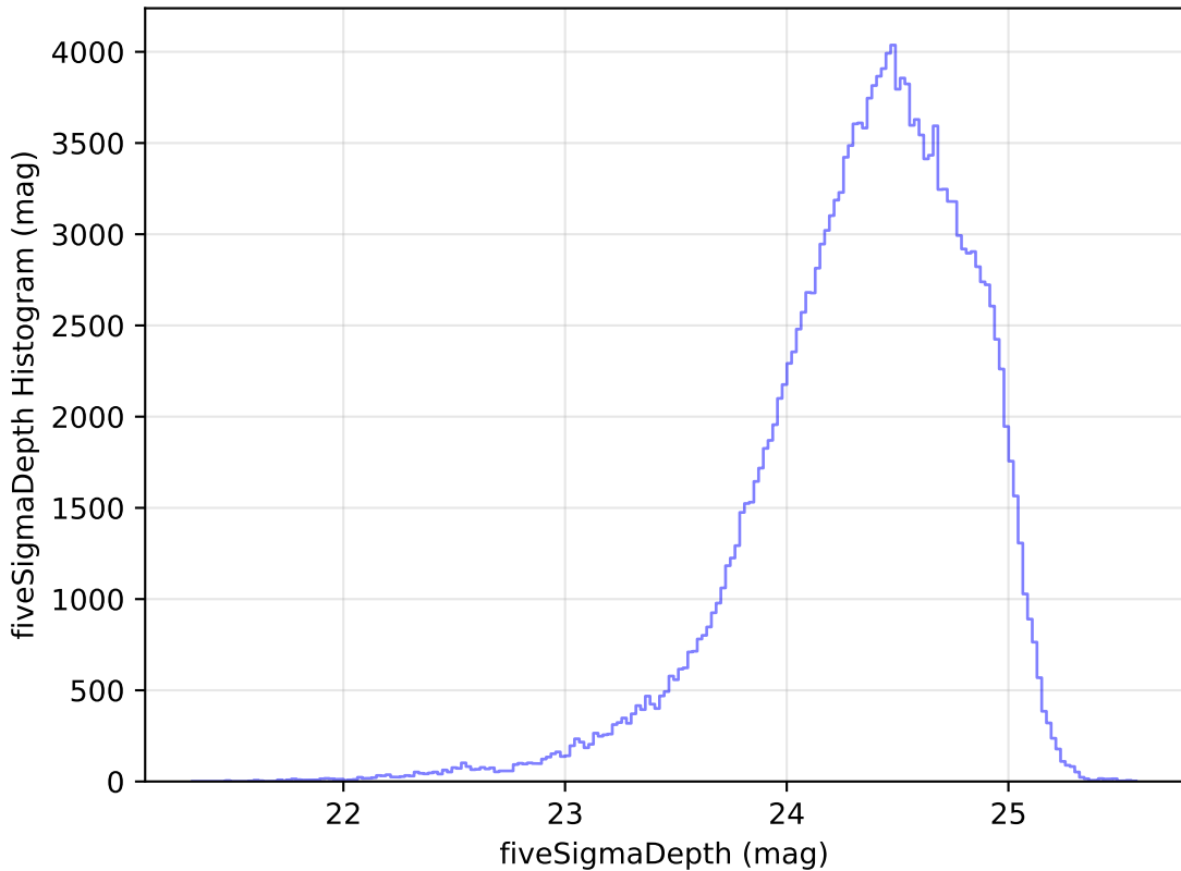
too_elab_r16_d3_gz_v3.4_10yrs All sky g band: fiveSigmaDepth Histogram
