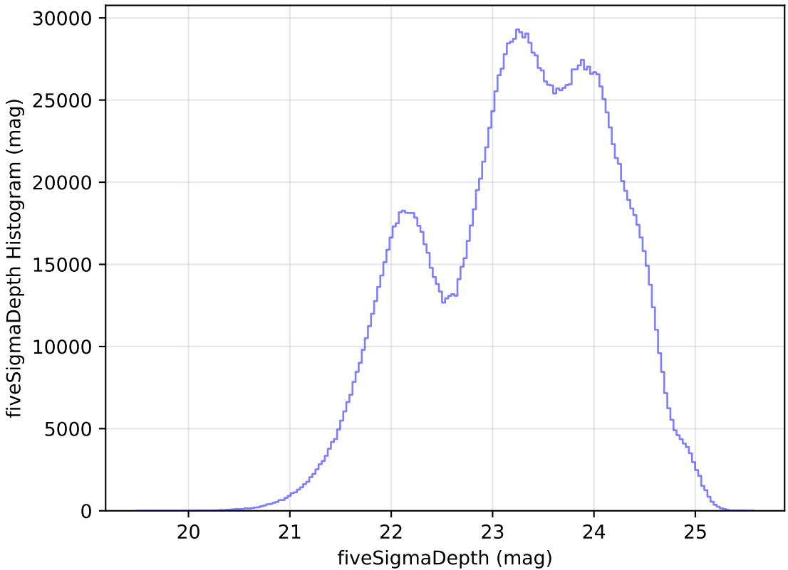
too_elab_r16_d3_gz_v3.4_10yrs All sky all bands: fiveSigmaDepth Histogram
