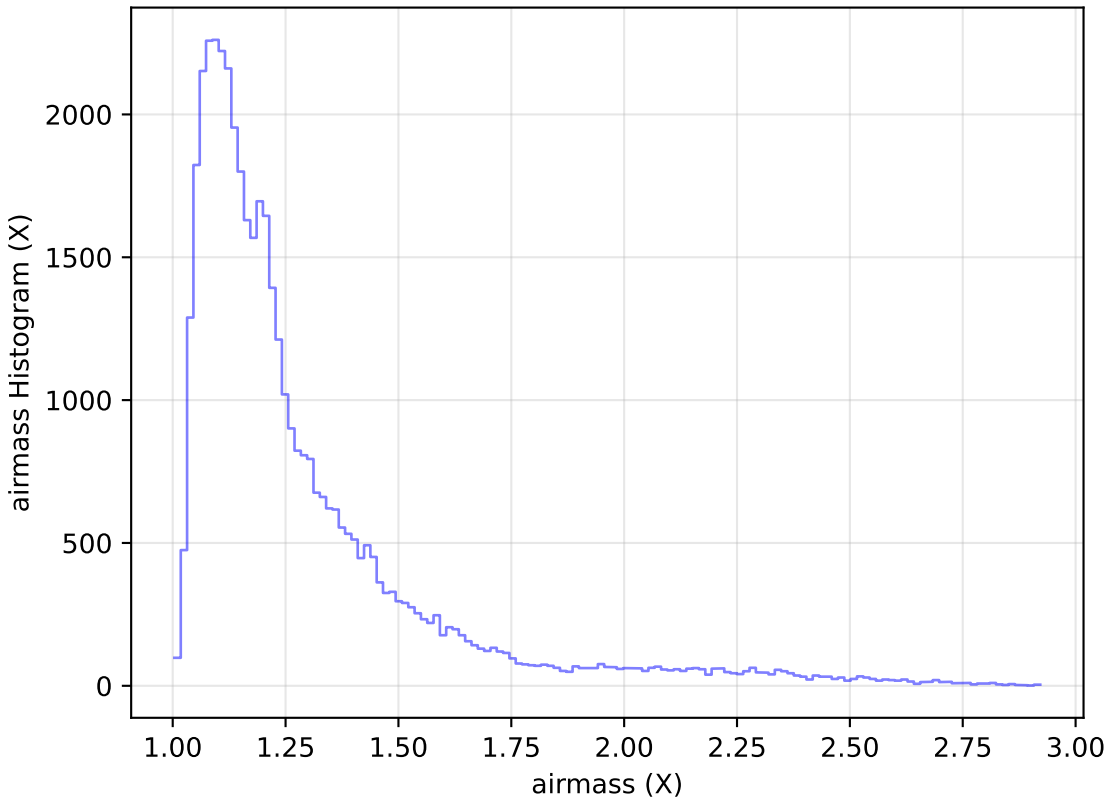
too_elab_r16_d3_gz_v3.4_10yrs Yr 1 z band: airmass Histogram
