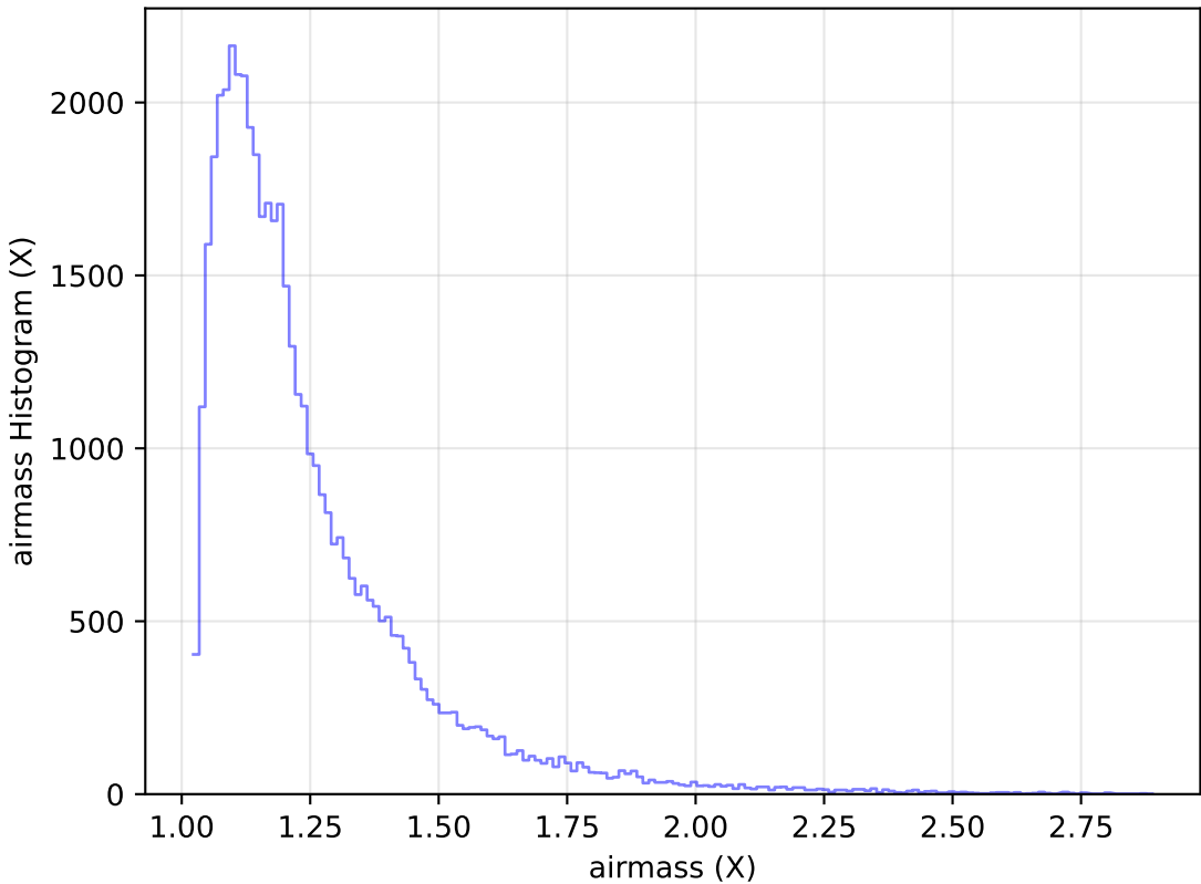
too_elab_r16_d3_gz_v3.4_10yrs Yr 1 y band: airmass Histogram
