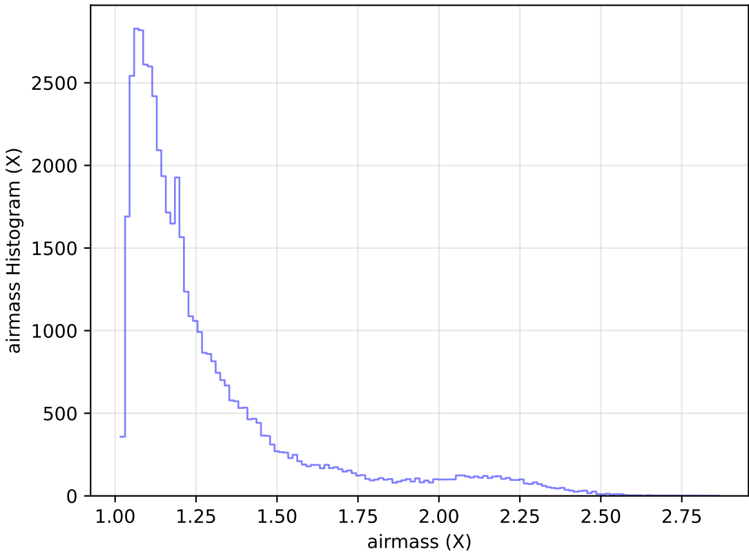
too_elab_r16_d3_gz_v3.4_10yrs Yr 1 r band: airmass Histogram
