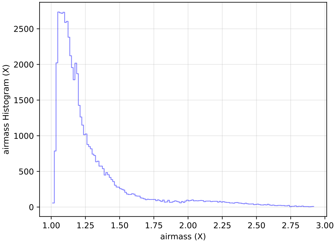
too_elab_r16_d3_gz_v3.4_10yrs Yr 1 i band: airmass Histogram
