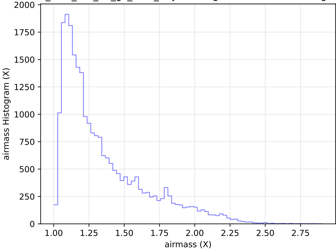
too_elab_r16_d3_gz_v3.4_10yrs Yr 1 g band: airmass Histogram
