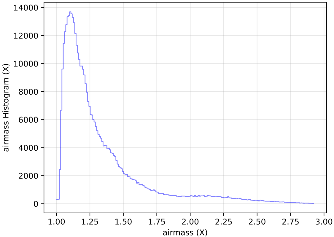
too_elab_r16_d3_gz_v3.4_10yrs WFD z band: airmass Histogram
