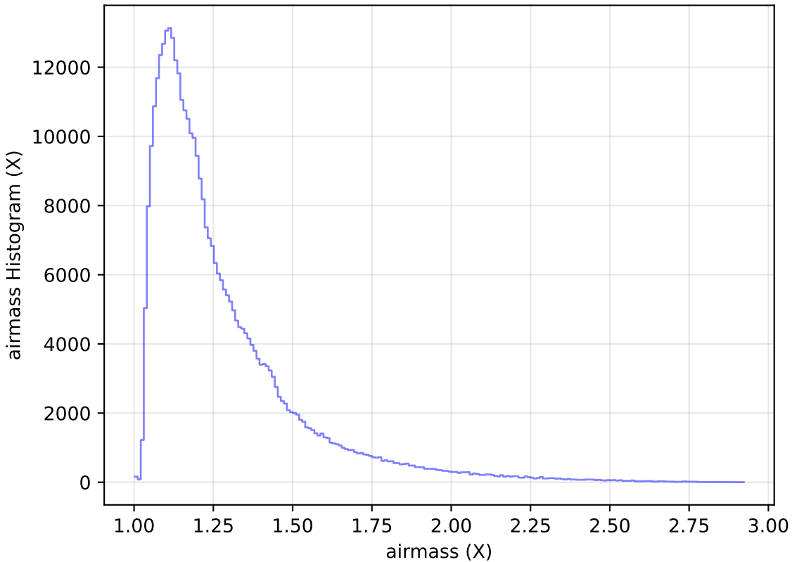
too_elab_r16_d3_gz_v3.4_10yrs WFD y band: airmass Histogram
