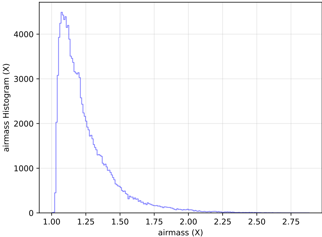
too_elab_r16_d3_gz_v3.4_10yrs WFD u band: airmass Histogram
