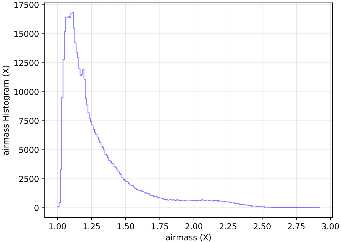
too_elab_r16_d3_gz_v3.4_10yrs WFD r band: airmass Histogram
