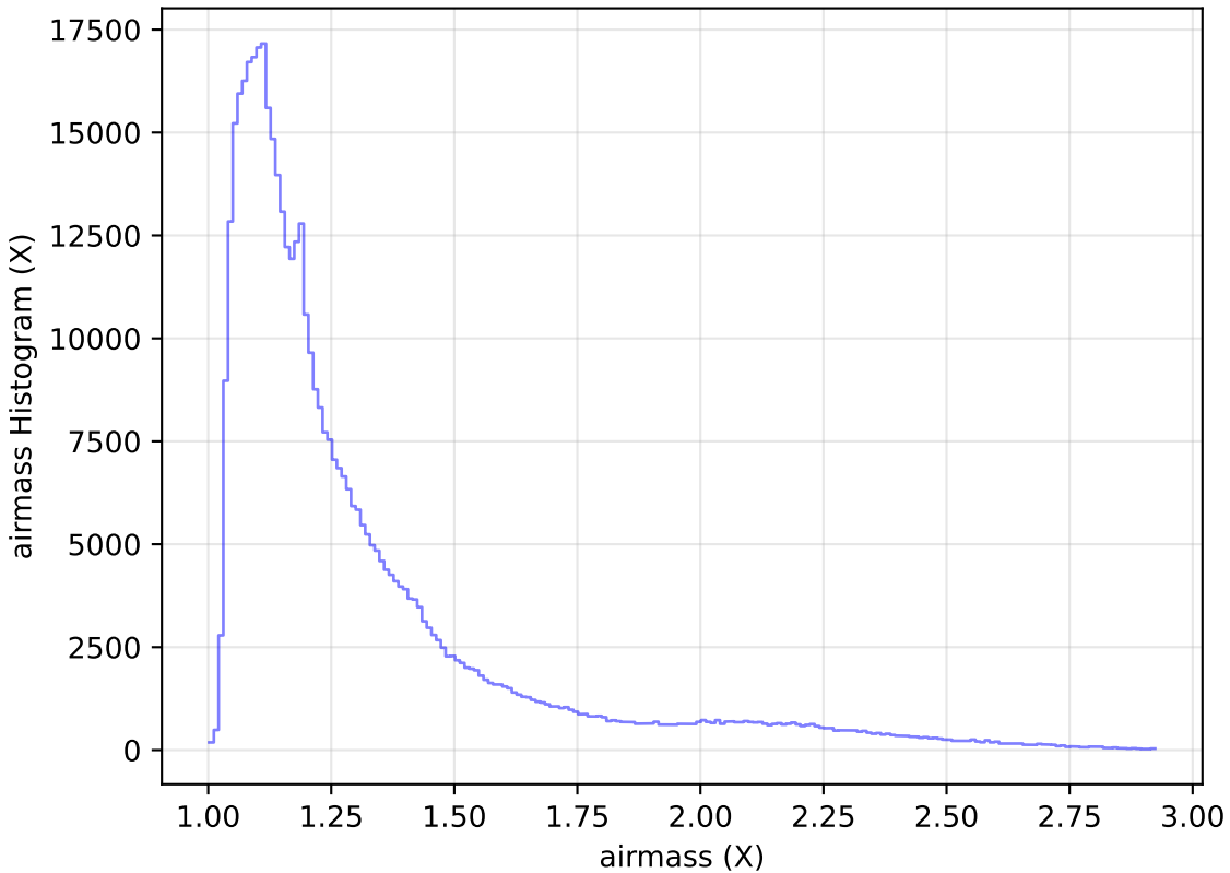
too_elab_r16_d3_gz_v3.4_10yrs WFD i band: airmass Histogram
