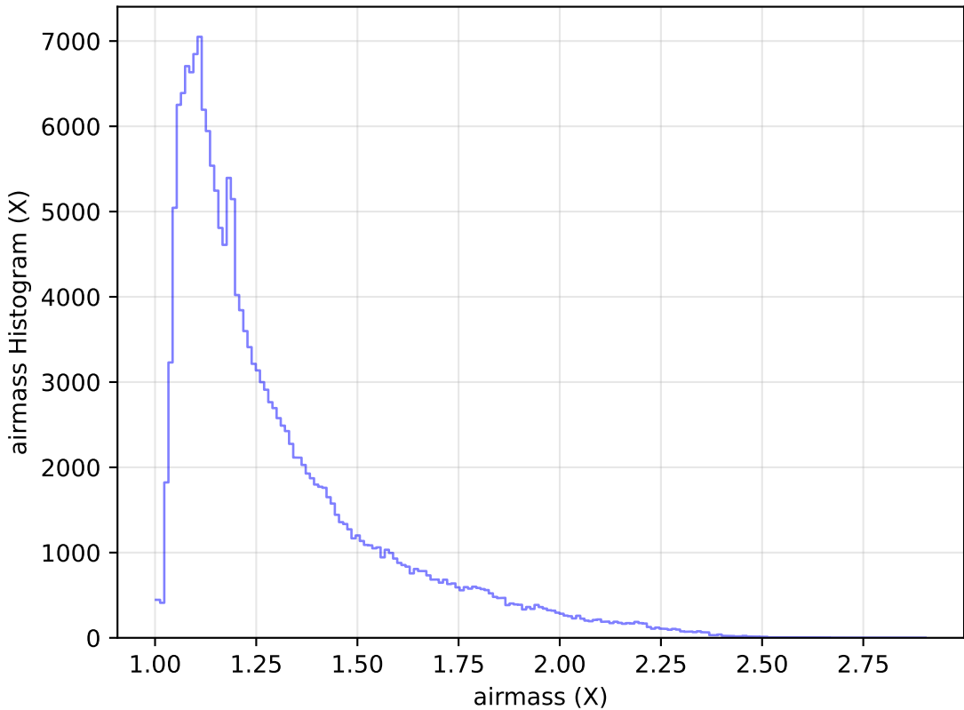
too_elab_r16_d3_gz_v3.4_10yrs WFD g band: airmass Histogram
