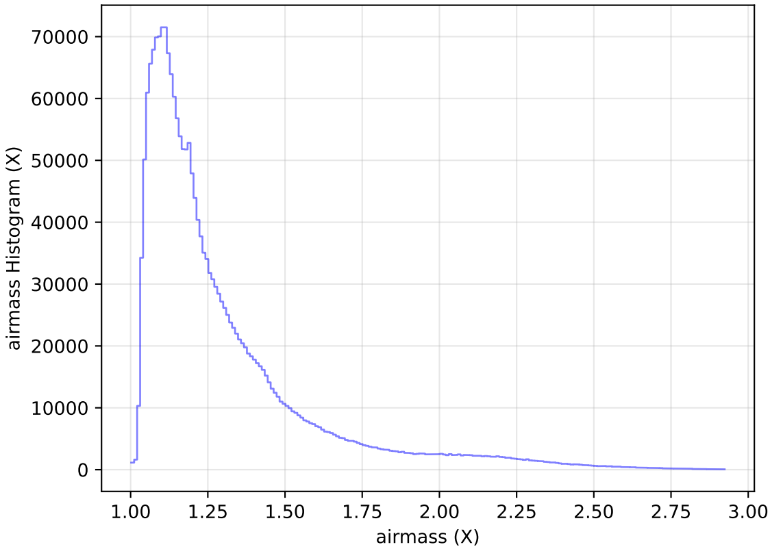
too_elab_r16_d3_gz_v3.4_10yrs WFD all bands: airmass Histogram
