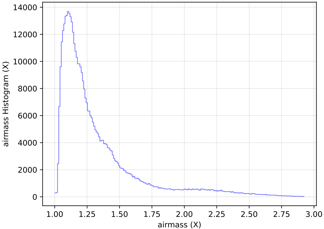
too_elab_r16_d3_gz_v3.4_10yrs All sky z band: airmass Histogram
