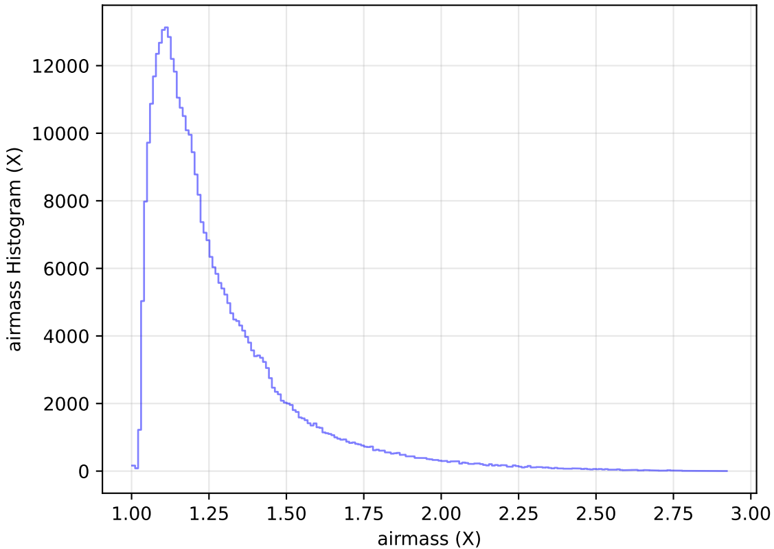
too_elab_r16_d3_gz_v3.4_10yrs All sky y band: airmass Histogram
