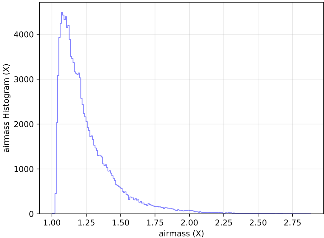
too_elab_r16_d3_gz_v3.4_10yrs All sky u band: airmass Histogram
