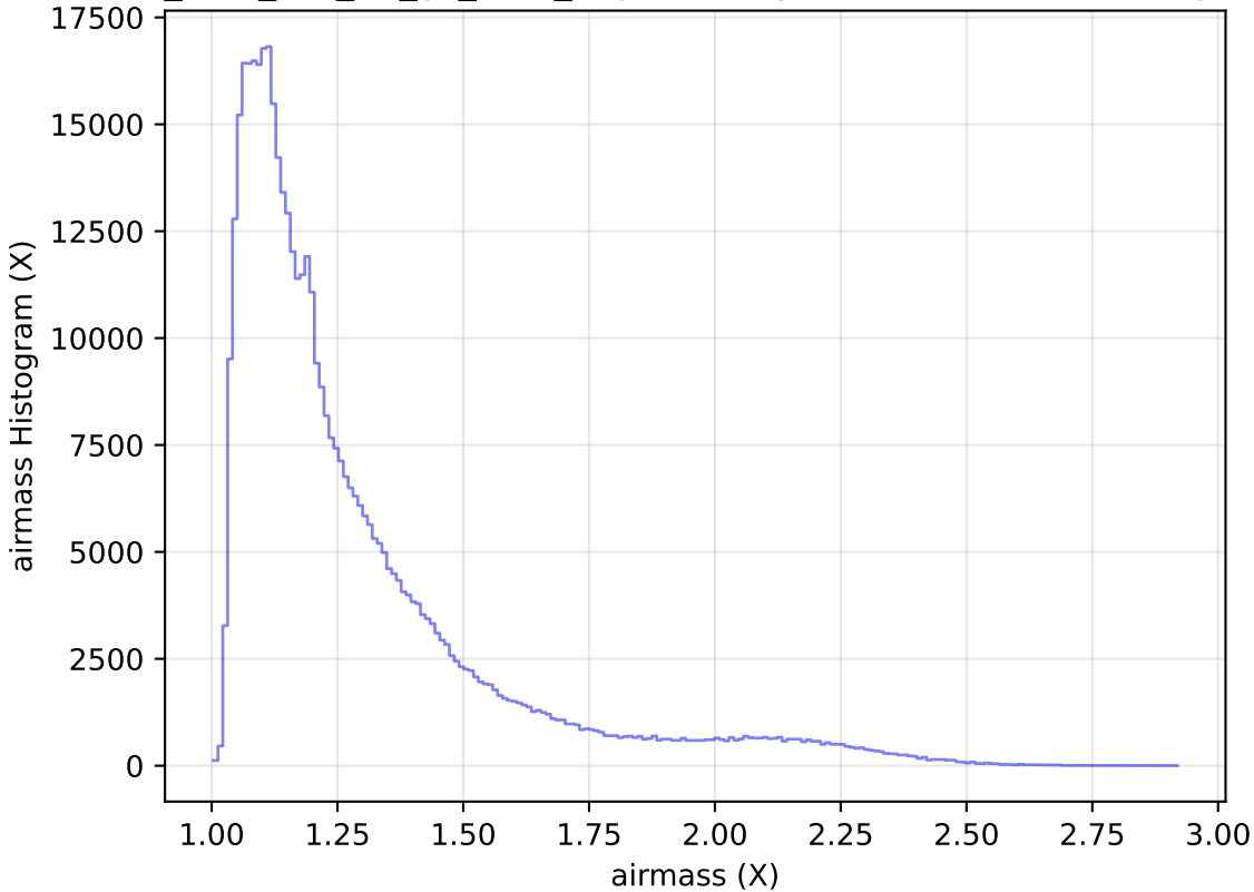
too_elab_r16_d3_gz_v3.4_10yrs All sky r band: airmass Histogram
