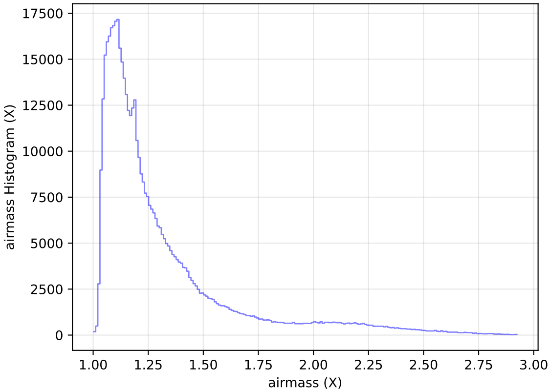
too_elab_r16_d3_gz_v3.4_10yrs All sky i band: airmass Histogram
