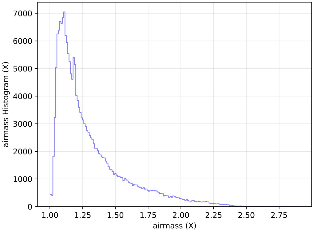
too_elab_r16_d3_gz_v3.4_10yrs All sky g band: airmass Histogram
