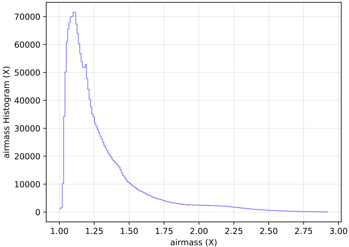
too_elab_r16_d3_gz_v3.4_10yrs All sky all bands: airmass Histogram
