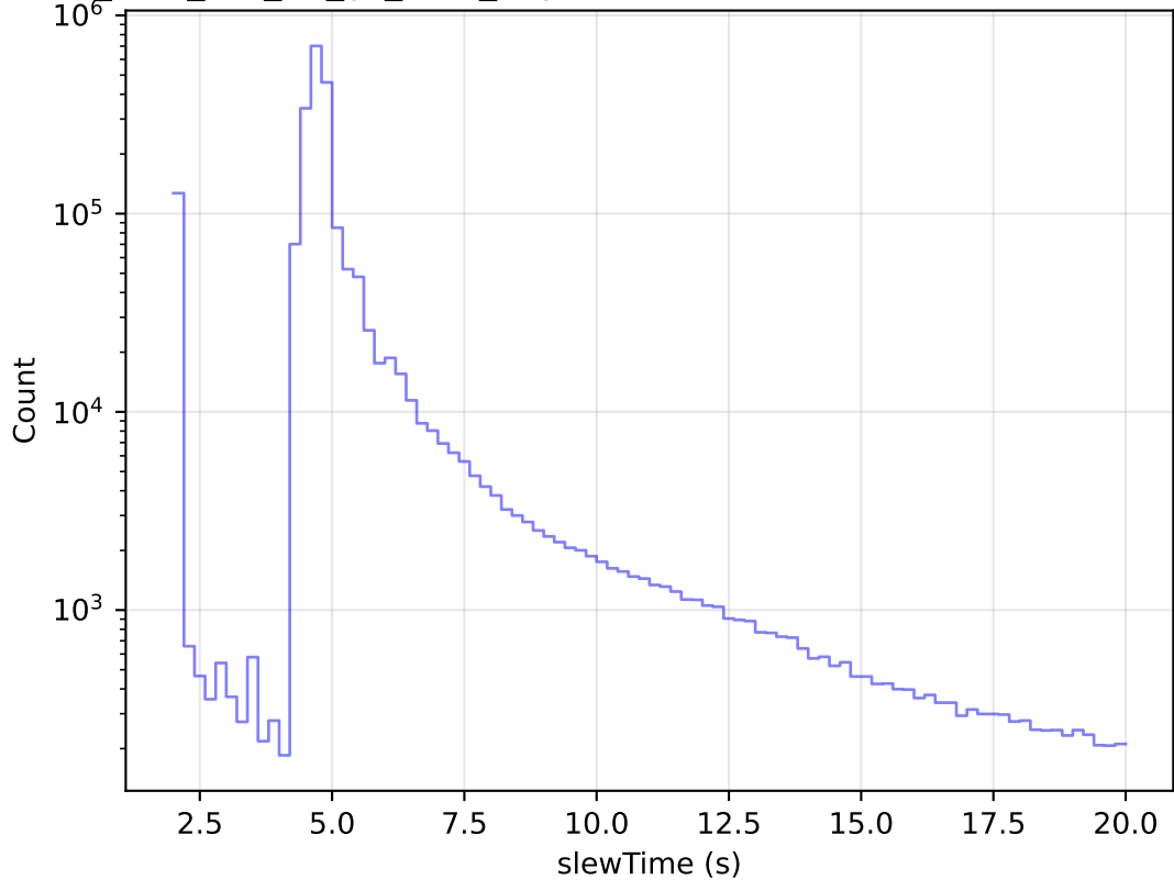
too_elab_r16_d3_gz_v3.4_10yrs All visits: Zoom Slew Time Histogram
