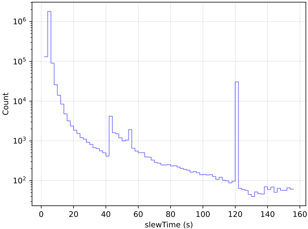
too_elab_r16_d3_gz_v3.4_10yrs All visits: Slew Time Histogram
