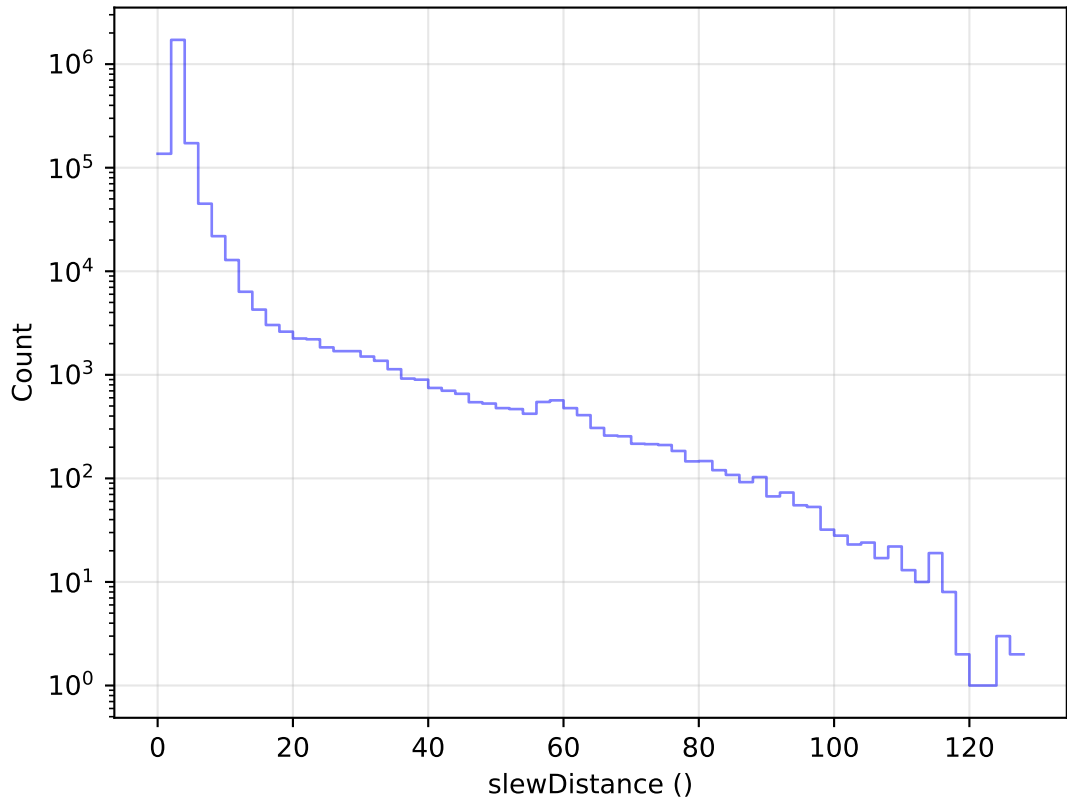
too_elab_r16_d3_gz_v3.4_10yrs All visits: Slew Distance Histogram
