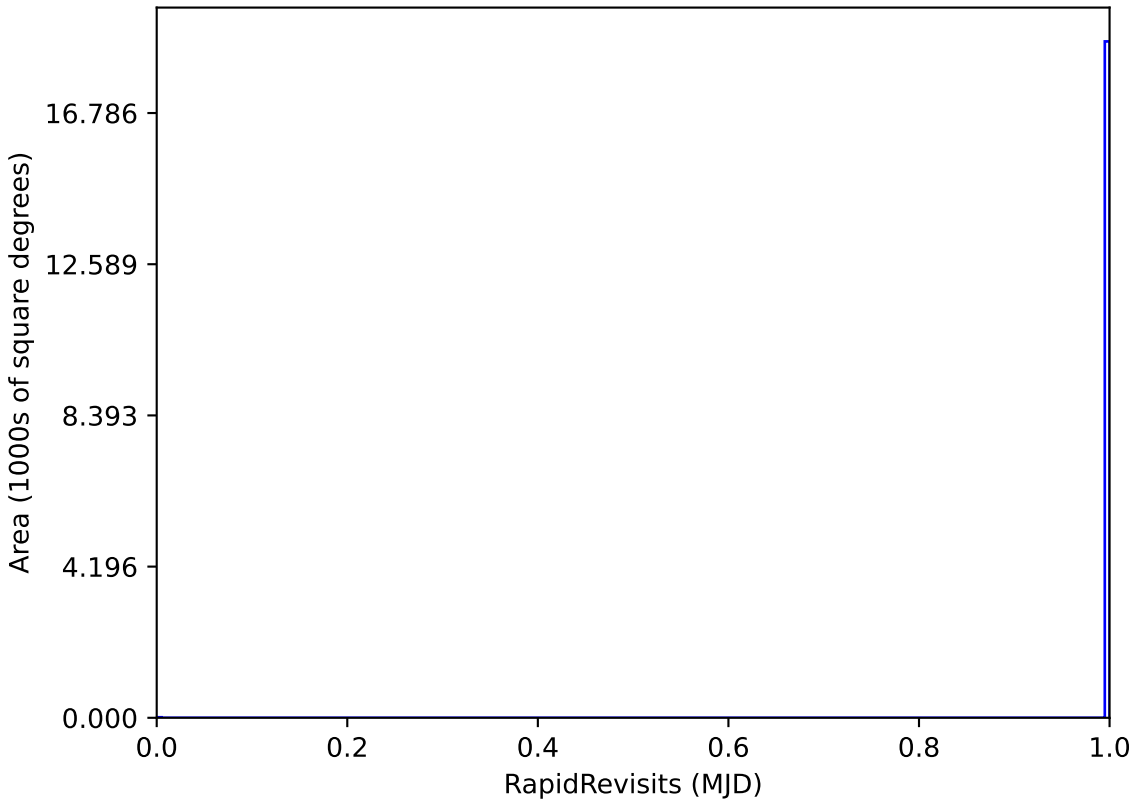
too_elab_r16_d3_gz_v3.4_10yrs WFD: RapidRevisits
