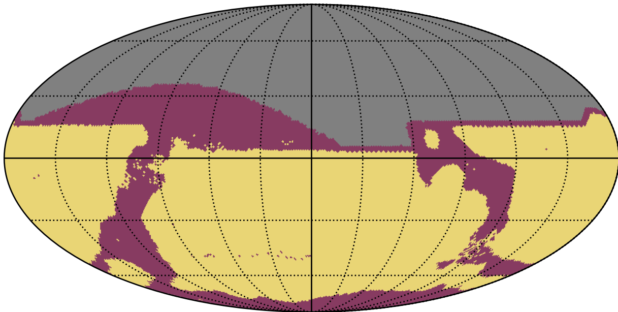
too_elab_r16_d3_gz_v3.4_10yrs All sky: RapidRevisits
