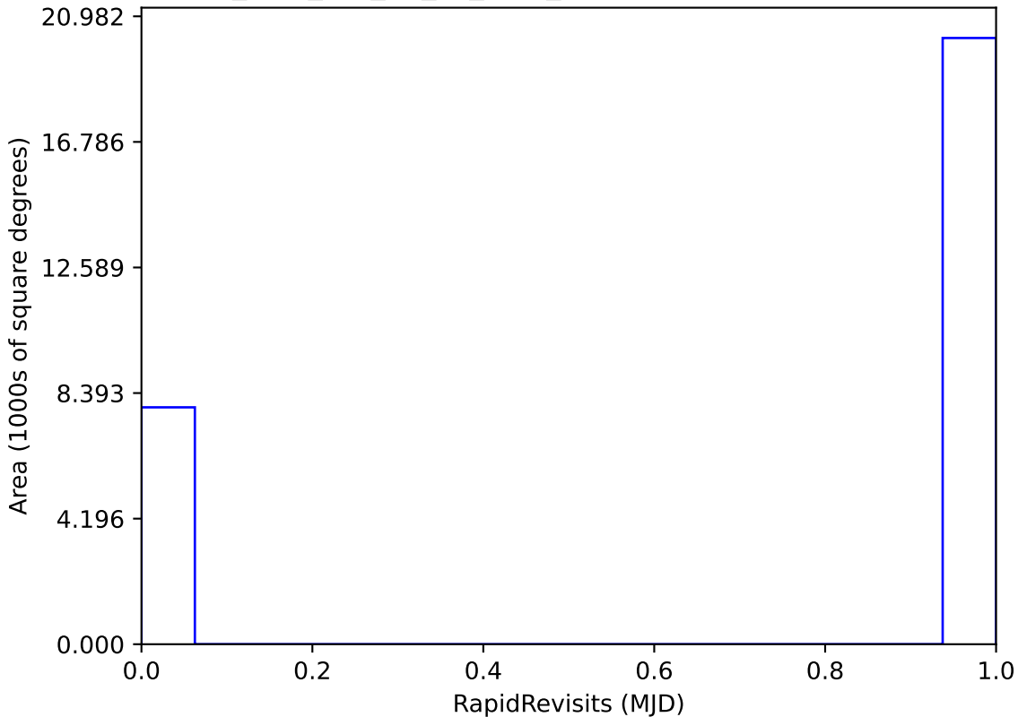
too_elab_r16_d3_gz_v3.4_10yrs All sky: RapidRevisits
