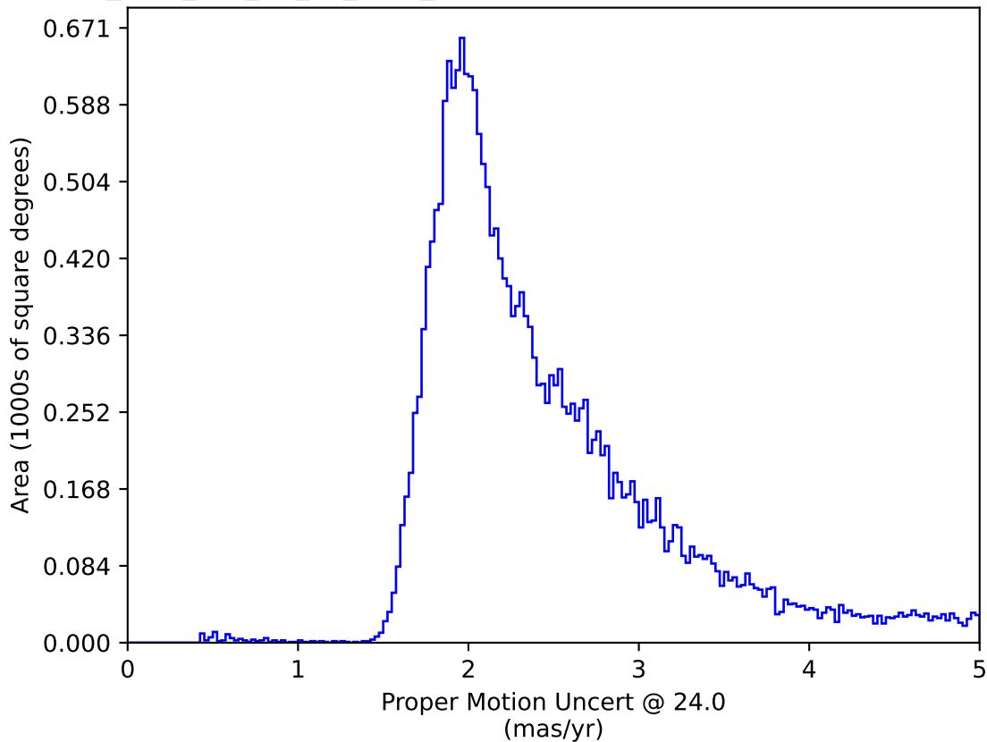
too_elab_r16_d3_gz_v3.4_10yrs All sky: Proper Motion Uncert @ 24.0
