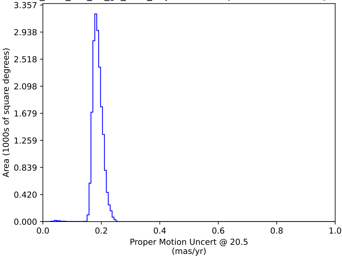
too_elab_r16_d3_gz_v3.4_10yrs WFD: Proper Motion Uncert @ 20.5
