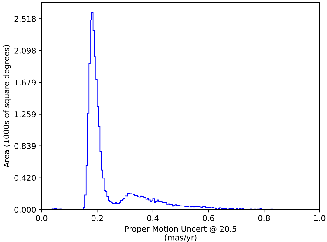
too_elab_r16_d3_gz_v3.4_10yrs All sky: Proper Motion Uncert @ 20.5
