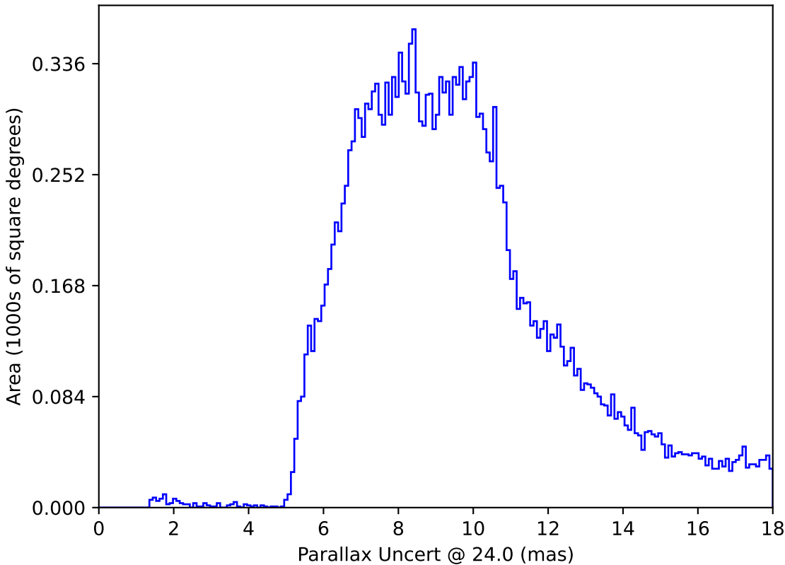
too_elab_r16_d3_gz_v3.4_10yrs All sky: Parallax Uncert @ 24.0
