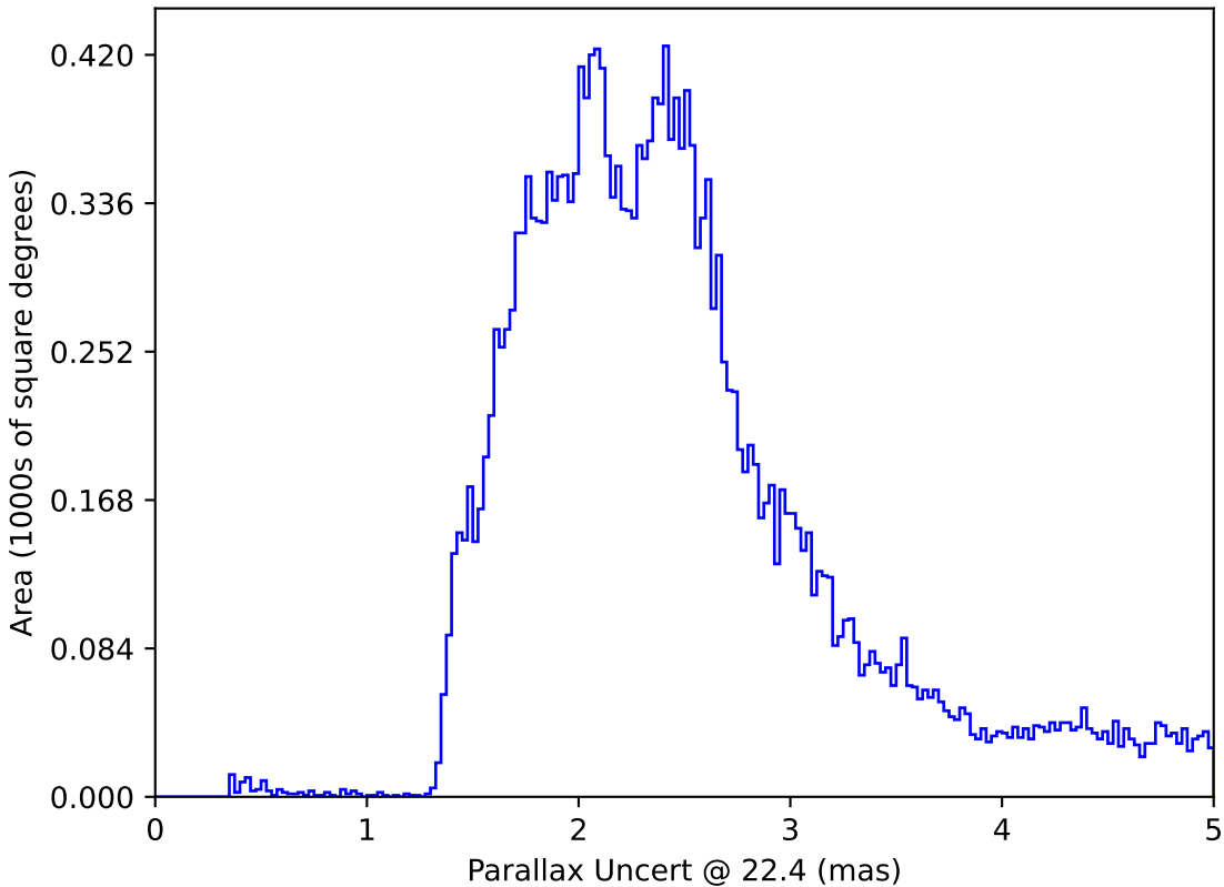
too_elab_r16_d3_gz_v3.4_10yrs All sky: Parallax Uncert @ 22.4
