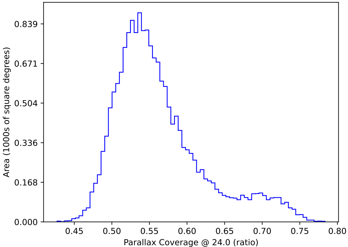
too_elab_r16_d3_gz_v3.4_10yrs WFD: Parallax Coverage @ 24.0
