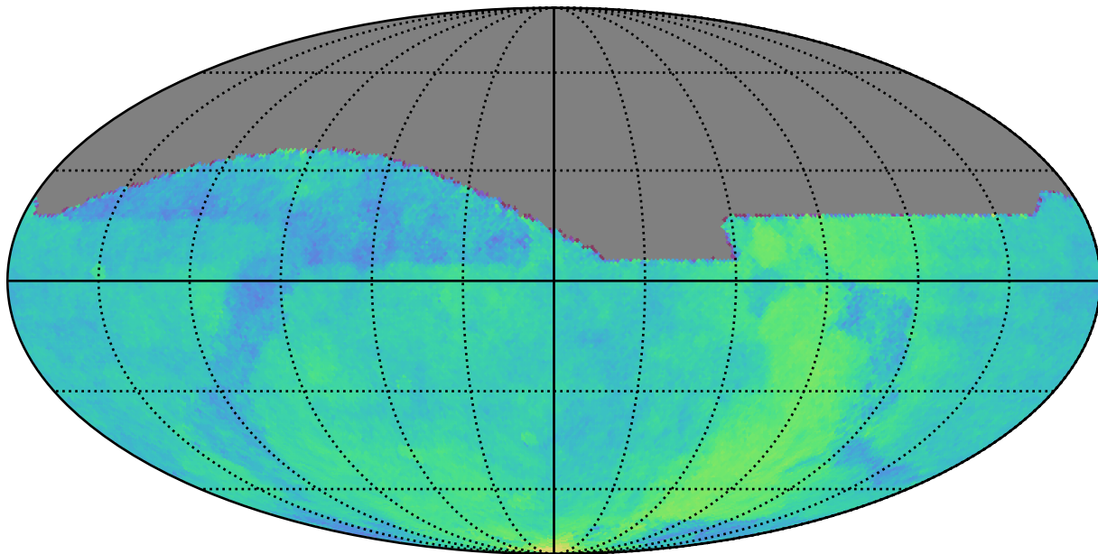
too_elab_r16_d3_gz_v3.4_10yrs All sky: Parallax Coverage @ 24.0
