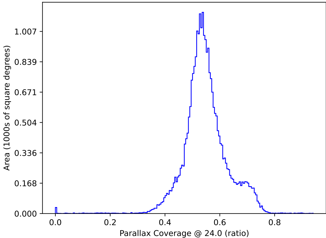
too_elab_r16_d3_gz_v3.4_10yrs All sky: Parallax Coverage @ 24.0
