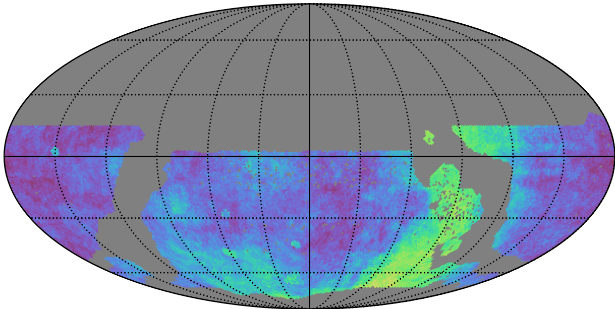
too_elab_r16_d3_gz_v3.4_10yrs WFD: Parallax Coverage @ 22.4
