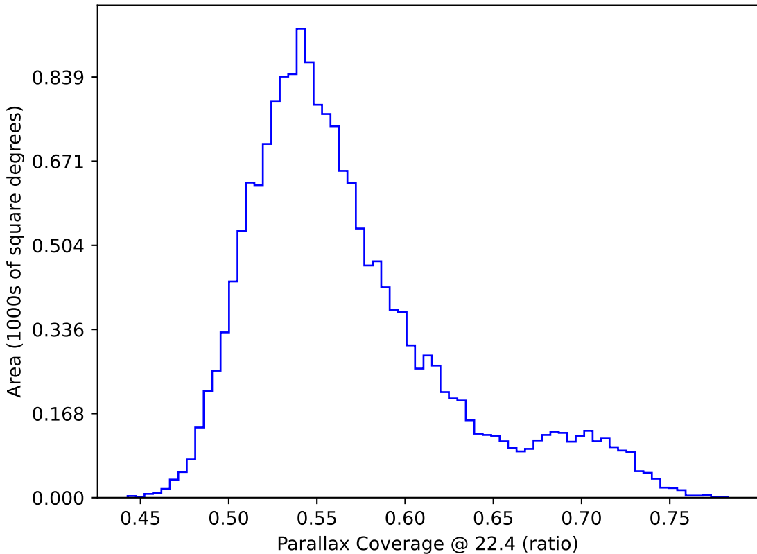
too_elab_r16_d3_gz_v3.4_10yrs WFD: Parallax Coverage @ 22.4
